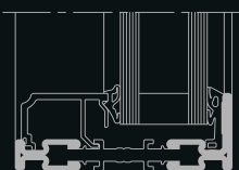
Glasleiste Kontur Contoured glazing bead
