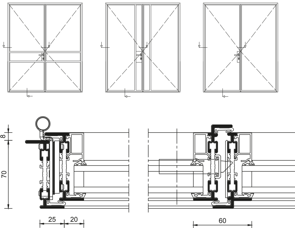
Tür 2-flügelig Two-leaf door
